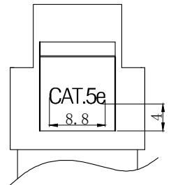
Long and short clip terminal
